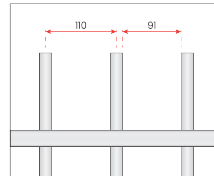
PICKET SPACING 110mm Centres | 91mm Airspace
