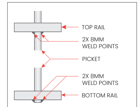
JOINT DETAILS Each Picket Welded to Rails with 2x 8mm Welds
