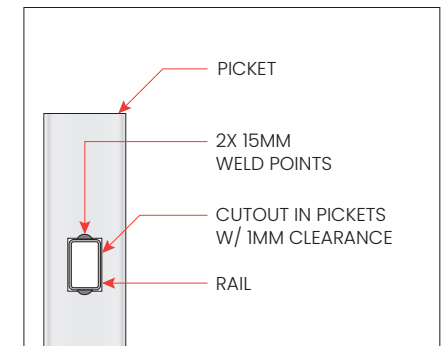
JOINT DETAILS
