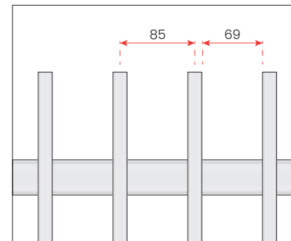
PICKET SPACING
