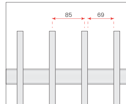
PICKET SPACING
