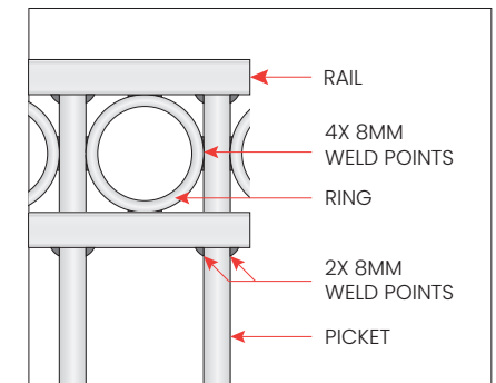
JOINT DETAILS
