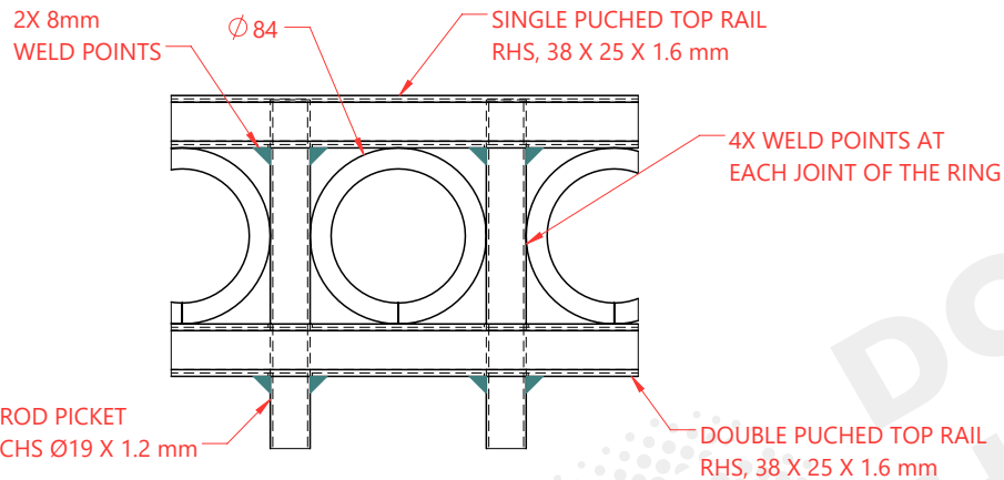
DETAIL A SCALE 1 : 4
