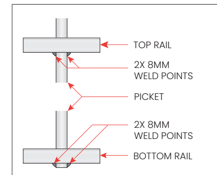
JOINT DETAILS Each Picket Welded to Rails with 2x 8mm Welds
