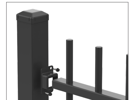
FIXING DETAILS
