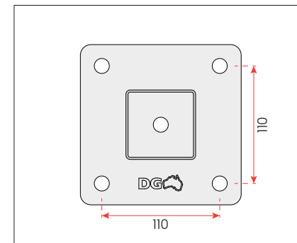
BASE PLATE DETAILS
