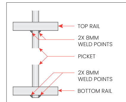
JOINT DETAILS
