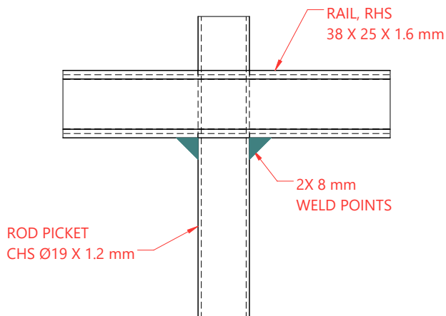
DETAIL A SCALE 1 : 2
