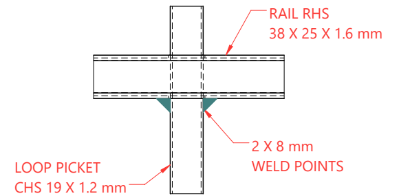
DETAIL A SCALE 1 : 3
