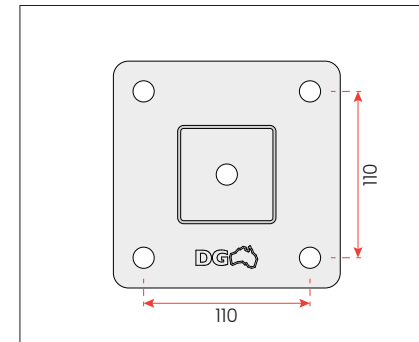
150 X 150 base plate with Ø14mm holes in 110 x 110 hole pattern
