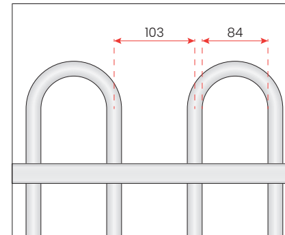
PICKET SPACING
