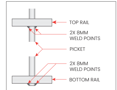
JOINT DETAILS
