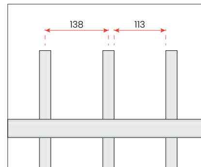
PICKET SPACING 138mm Centres | 113mm Airspace
