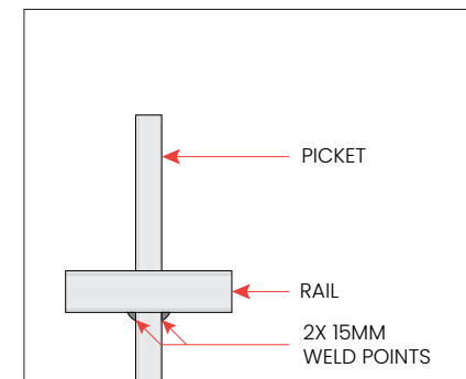
JOINT DETAILS Each Picket Welded to Rails with 2x 15mm Welds
