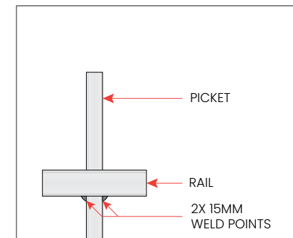
JOINT DETAILS
