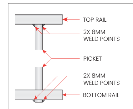
JOINT DETAILS
