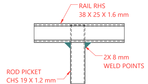
DETAIL B SCALE 1 : 3
