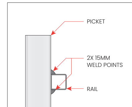
JOINT DETAILS
